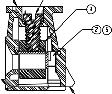
SECTION Z-Z ALIGNMENT FEATURE
