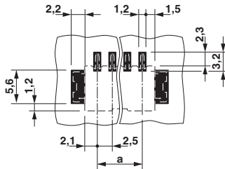
Drilling diagram
