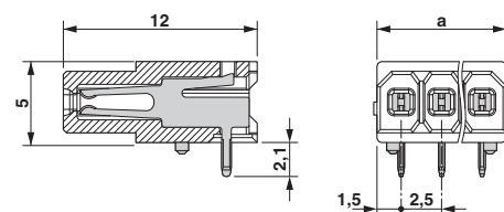
Dimensioned drawing
