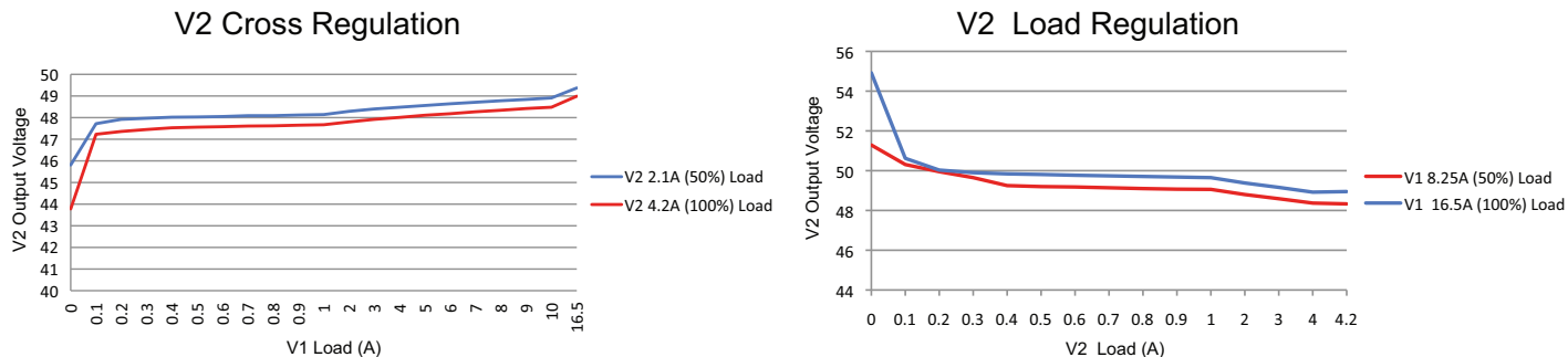
Figure 5 - EMH350PD24
