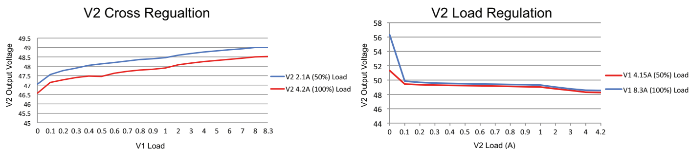
Figure 5 - EMH350PD24
