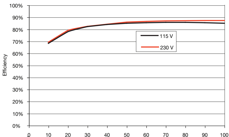
Figure 9 EMH350PS12
