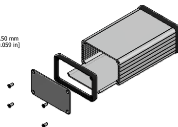
EXPLODED ASSEMBLY VIEW
