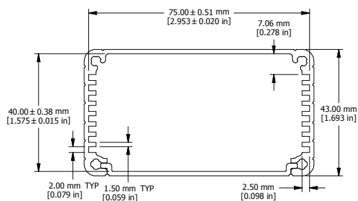
EXTRUSION
