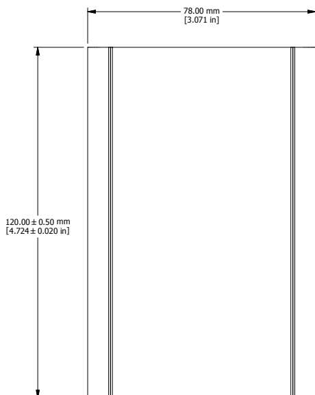
EXTRUSION
