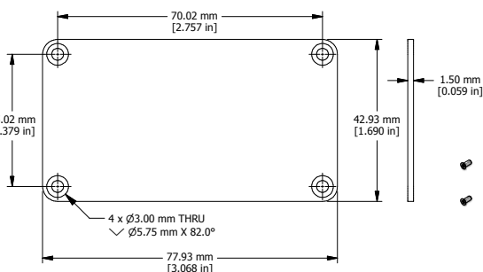
END PLATE
