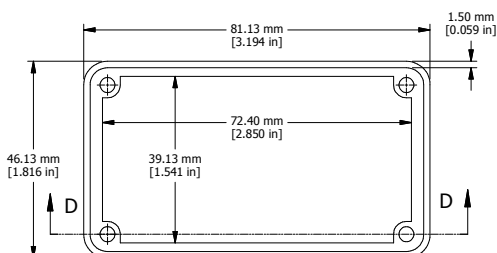
EXTRUSION DESIGNED FOR 75MM WIDE PC BOARD
