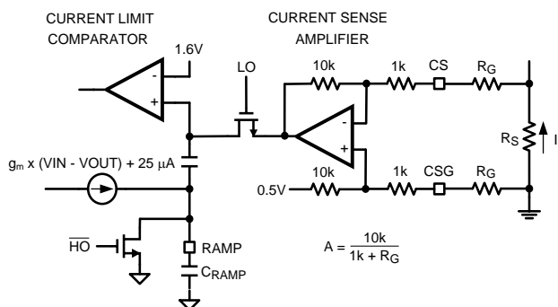
Figure 9. Current Limit and Ramp Circuit
