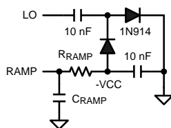
Figure 16. R RAMP to -VCC for V OUT < 7.5 V
