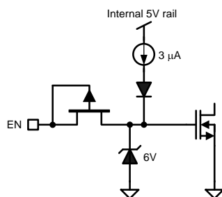
Figure 5. Enable Circuit
