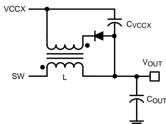
Figure 3. VCCX Bias Supply with Additional Inductor Winding
