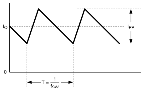
Figure 11. Inductor Current
