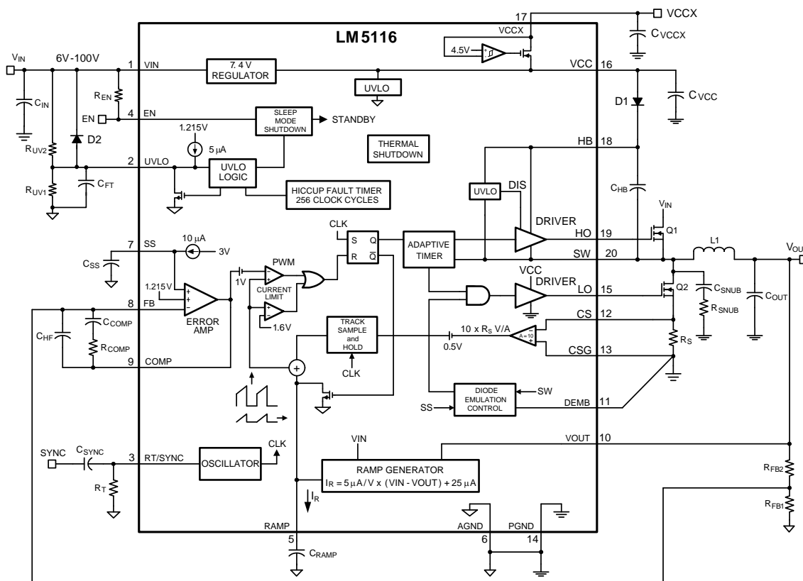
Figure 2. Typical Application
