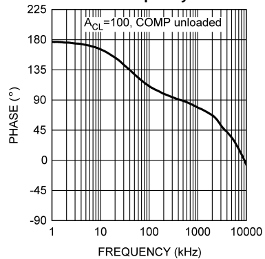
Error Amp Phase vs Frequency
