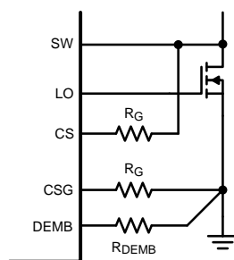
Figure 8. R_{DS(ON)} Current Sensing without Diode Emulation
