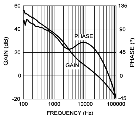
Figure 14. Overall Voltage Loop Gain and Phase
