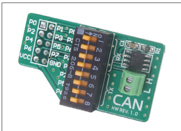
Figure 1: CAN additional board
