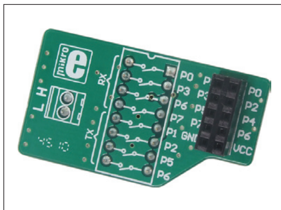
Figure 2: The back side of the CAN board
