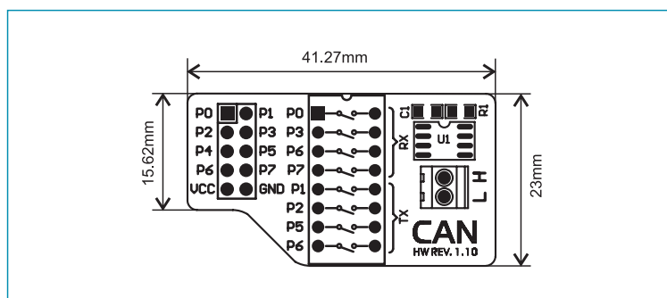
Figure 5: Dimensions of the additional board
