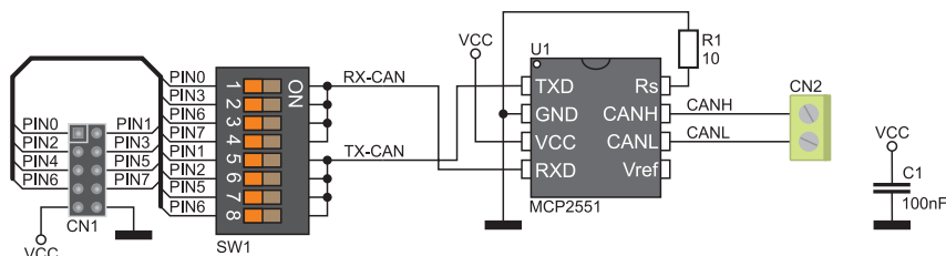
Figure 3: CAN additional board connection schematic
