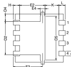
Backside view of single pad
