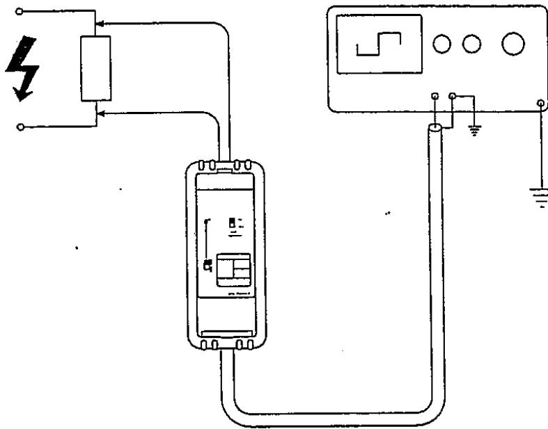
Differential probe for safe measurements
