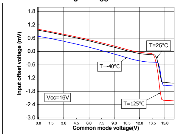
Figure 8. Input offset voltage vs. common mode voltage at V_{CC} = 16\text{ V}
