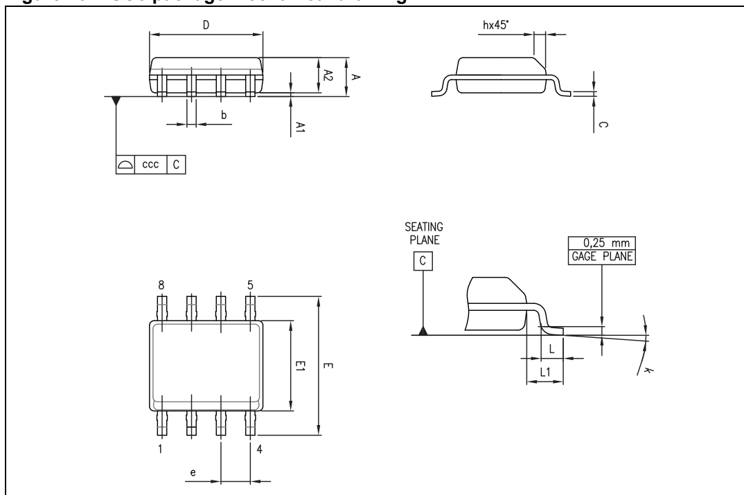
Figure 46. SO8 package mechanical drawing
