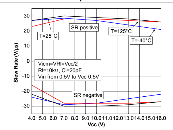
Figure 21. Slew rate vs. supply voltage and temperature
