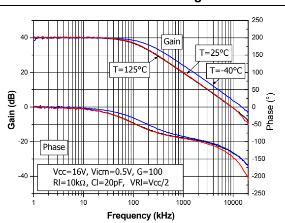
Figure 17. Bode diagram at V_{CC} = 16\text{ V} with low common mode voltage
