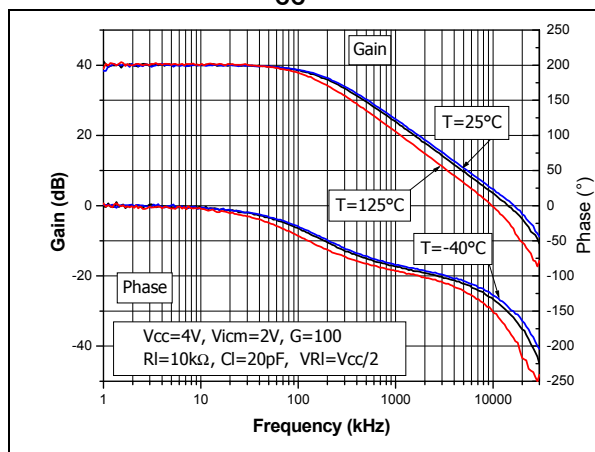
Figure 14. Bode diagram vs. temperature for V_{CC} = 4\text{ V}
