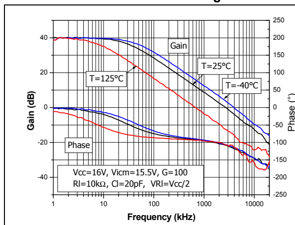
Figure 18. Bode diagram at V_{CC} = 16\text{ V} with high common mode voltage
