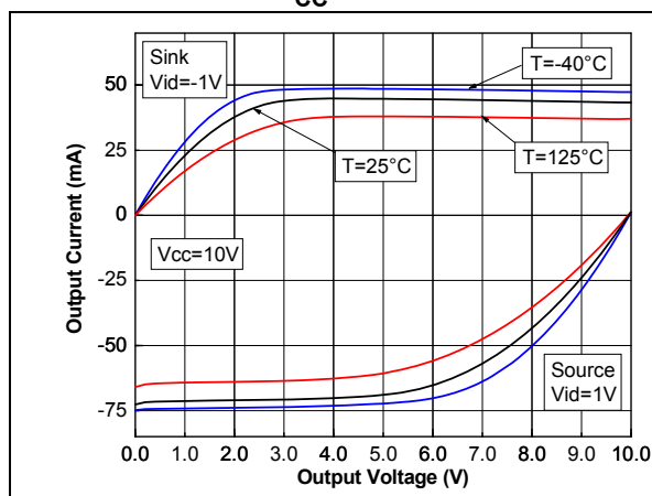
Figure 10. Output current vs. output voltage at V_{CC} = 10\text{ V}
