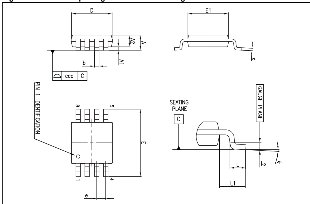
Figure 45. MiniSO8 package mechanical drawing
