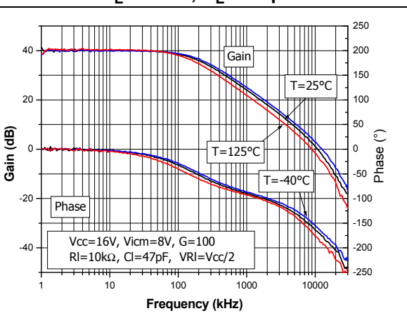
Figure 19. Bode diagram at V_{CC} = 16\text{ V} and R_L = 10\text{ k}\Omega , C_L = 47\text{ pF}
