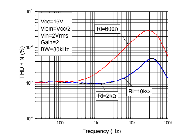
Figure 31. THD+N vs. frequency at VCC = 16 V
