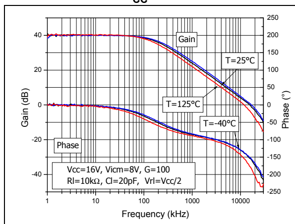
Figure 16. Bode diagram vs. temperature for V_{CC} = 16\text{ V}
