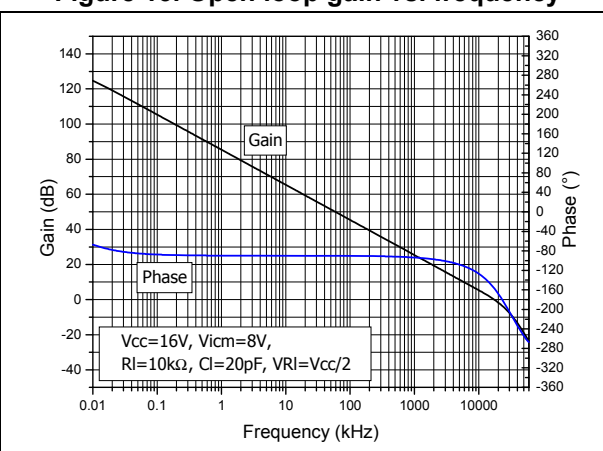
Figure 13. Open loop gain vs. frequency
