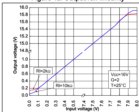
Figure 12. Output rail linearity
