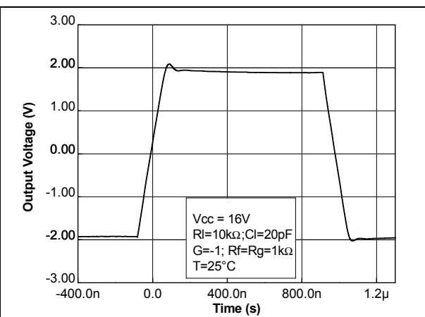
Figure 25. Large step response
