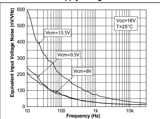
Figure 29. Noise vs. frequency with 16 V supply voltage
