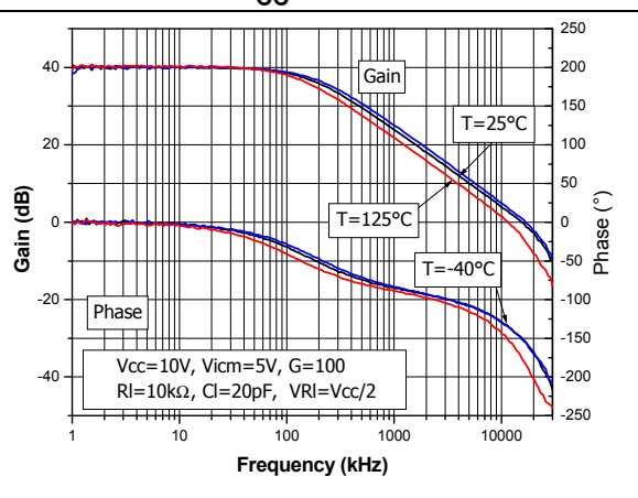
Figure 15. Bode diagram vs. temperature for V_{CC} = 10\text{ V}
