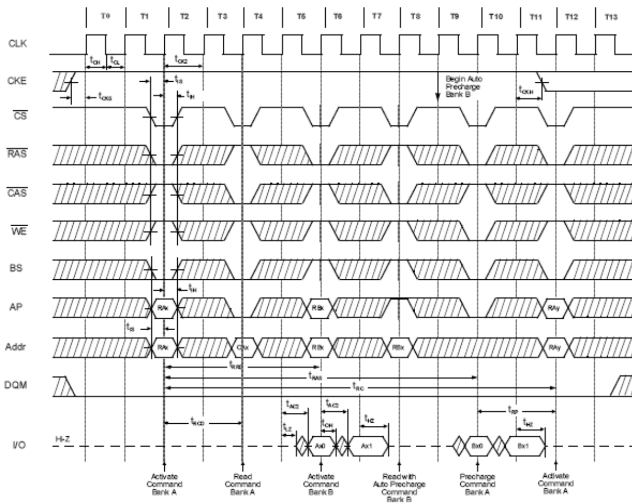
9.2 AC Parameters for Read Timing
