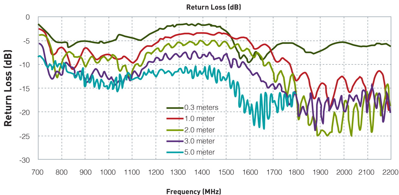
Figure 4. Return loss of MA520 Cellular Antenna on 60 *60 cm metal plate.
