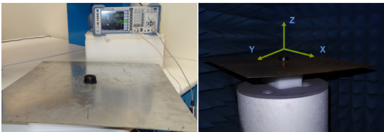
Figure 1. Impedance measurement (left hand) and efficiency and radiation pattern measurements (right hand).
