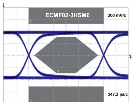
Figure 12. USB2.0 480 Mbps eye diagram with device
