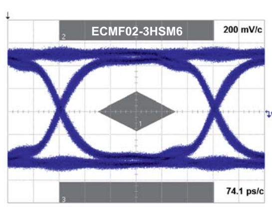
Figure 16. MHL 2.25 Mbps eye diagram with device
