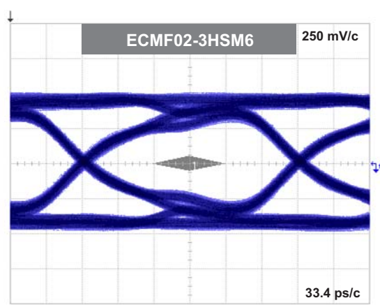
Figure 14. USB3.0 5 Gbps eye diagram with device
