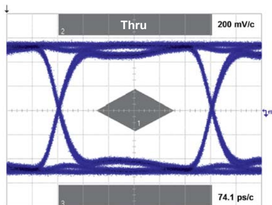
Figure 15. MHL 2.25 Mbps eye diagram without device
