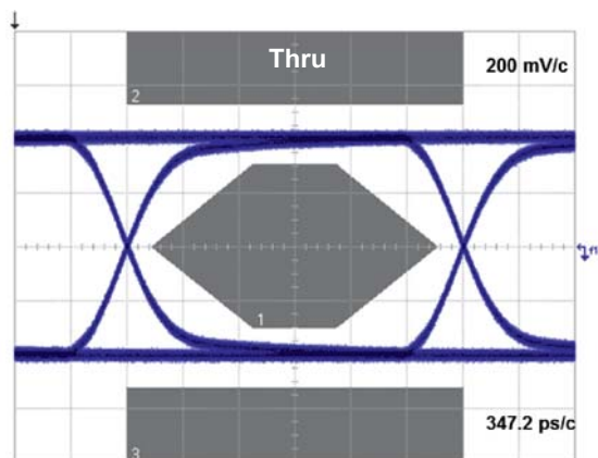
Figure 11. USB2.0 480 Mbps eye diagram without device
