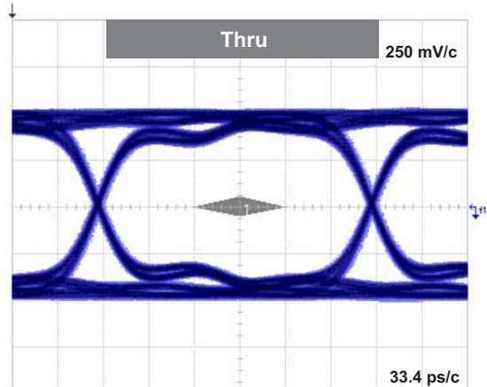
Figure 13. USB3.0 5 Gbps eye diagram without device
