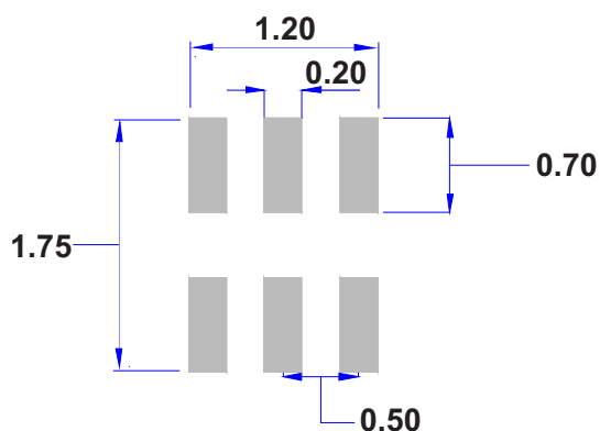
Figure 22. Footprint
