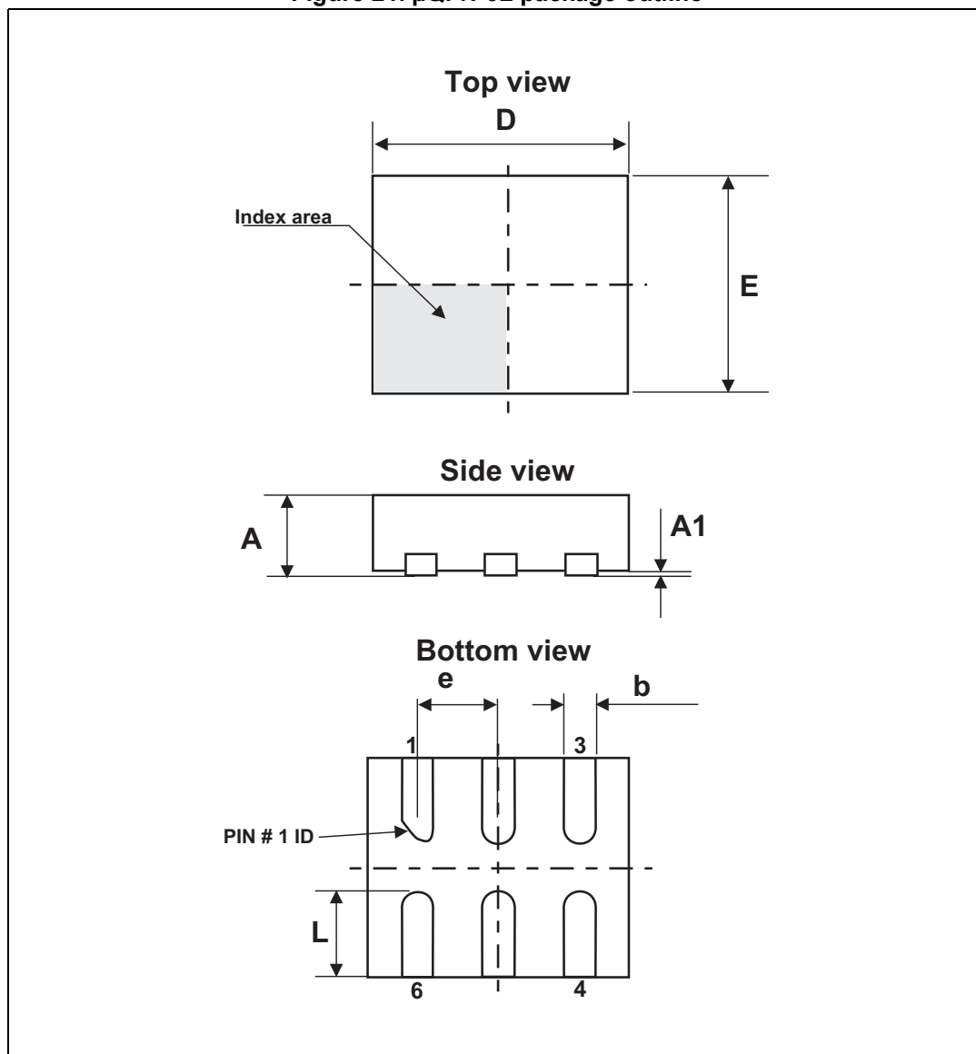
Figure 21. \mu QFN-6L package outline
