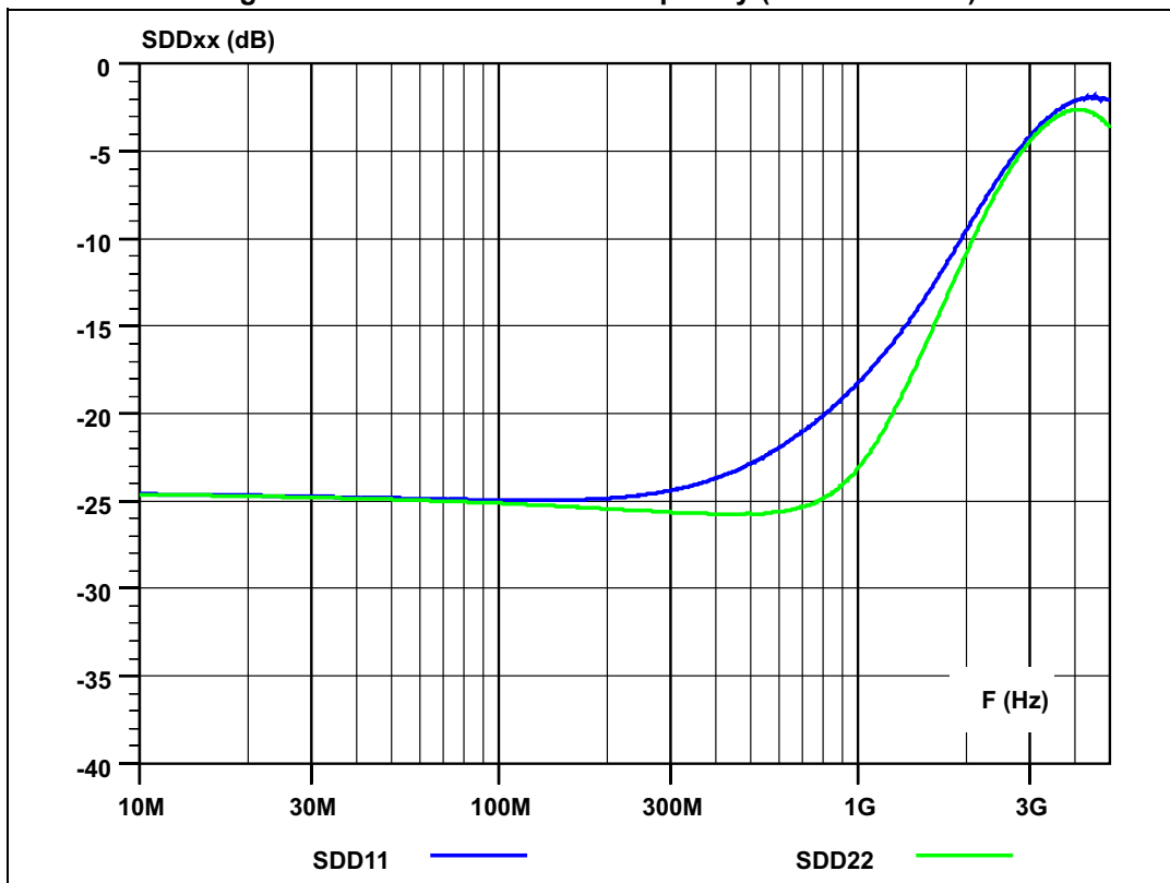
Figure 5. Return loss versus frequency ( Z_0 com = 50 \Omega )
