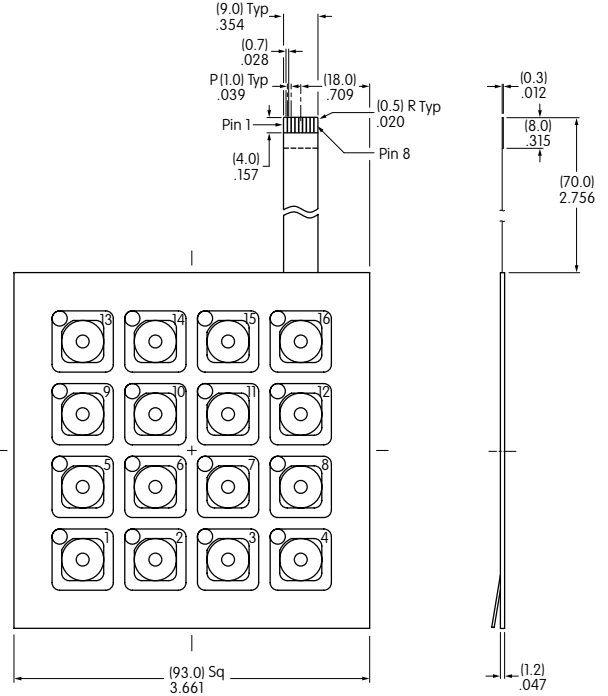
Switch Circuit Matrix Detail For 4 or 16 Key
