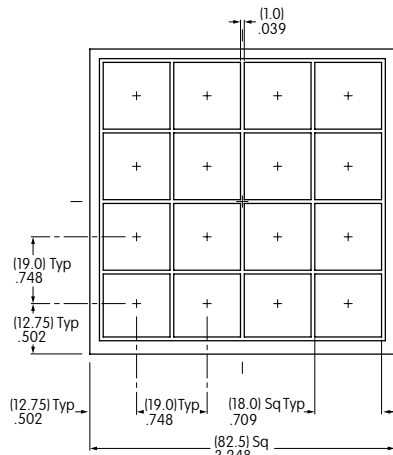
Insertable Legend Card for 4 Key or 16 Key
