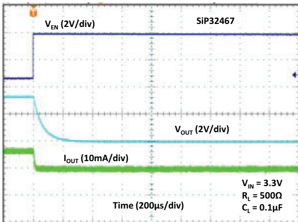
Fig. 29 - Turn-off Time
