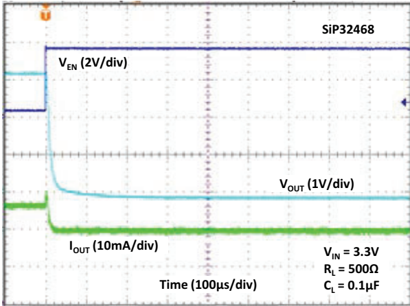
Fig. 34 - Turn-off Time
