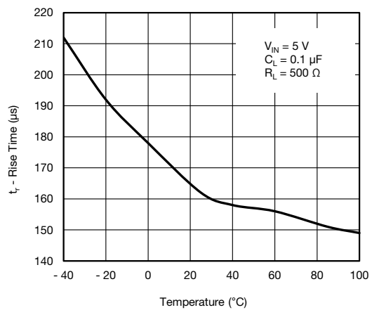
Fig. 15 - Rise Time vs. Temperature
