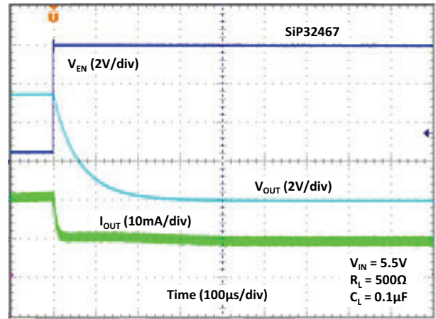
Fig. 31 - Turn-off Time
