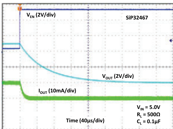
Fig. 30 - Turn-off Time
