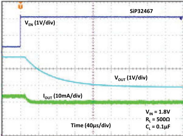
Fig. 28 - Turn-off Time
