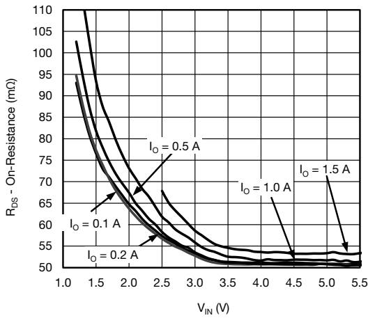
Fig. 11 - R_{DS(on)} vs. Input Voltage
