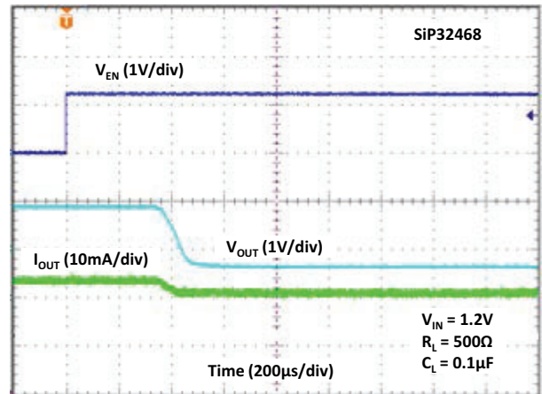
Fig. 32 - Turn-off Time
