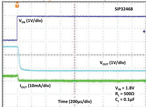
Fig. 33 - Turn-off Time
