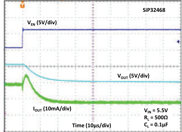
Fig. 36 - Turn-off Time
