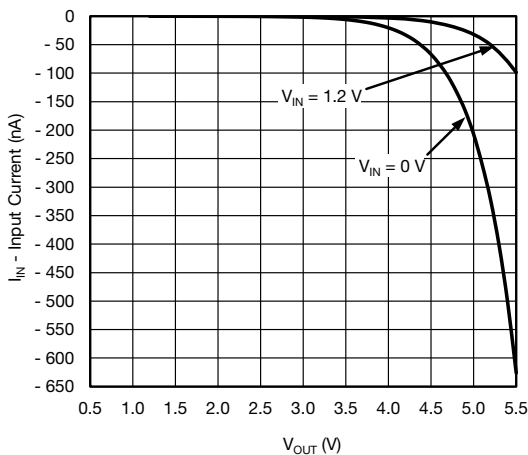
Fig. 12 - Reverse Blocking Current vs. Output Voltage
