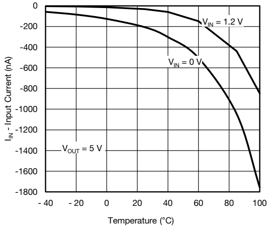
Fig. 16 - Reverse Blocking Current vs. Temperature
