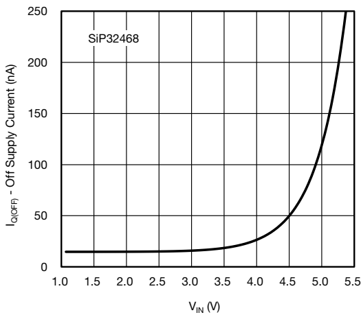
Fig. 5 - Off Supply Current vs. Input Voltage
