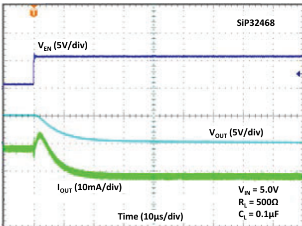
Fig. 35 - Turn-off Time
