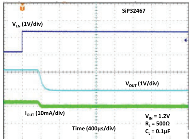
Fig. 27 - Turn-off Time
