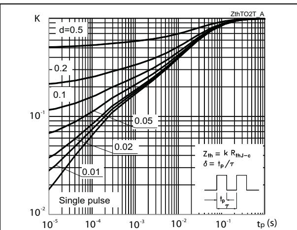
Figure 21. Thermal impedance
