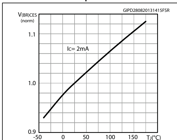
Figure 10. Normalized V_{(BR)CES} vs. junction temperature
