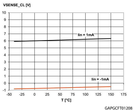
Figure 33. V_{\text{sense clamp}} vs. T_{\text{case}}
