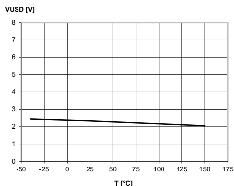
Figure 24. Undervoltage shutdown
