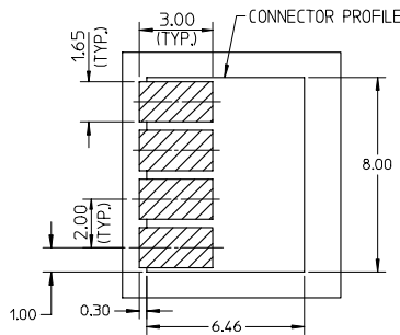
RECOMMENDED FOOT PRINT
