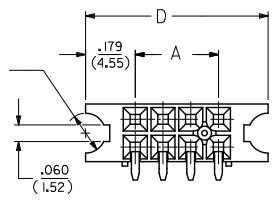
OPTION "H" ASSEMBLY STD. HOUSING W/MOUNTING EARS AND LOWER PINSTOP SCALE 4:1
