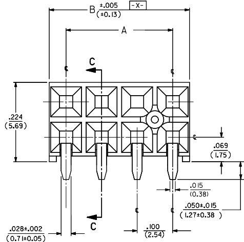
OPTION "C" ASSEMBLY STANDARD HOUSING
