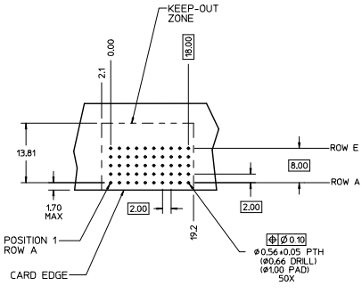
DAUGHTERCARD HOLE PATTERN (CONNECTOR SIDE)
