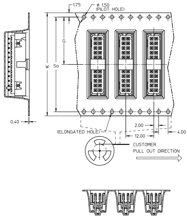
EMBOSSED CARRIER TAPE LAYOUT 24 CKT USE FOR ILLUSTRATION ONLY
