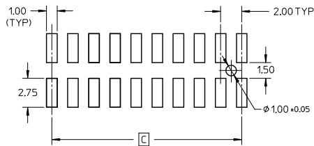
RECOMMENDED PCB PATTERN
