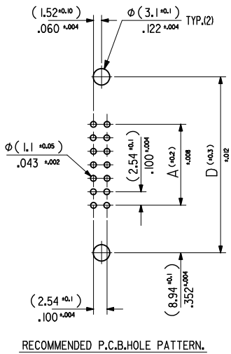
RECOMMENDED P.C.B. HOLE PATTERN.
