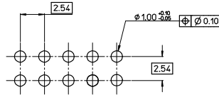
RECOMENDEC P.C. BOARD HOLE PATTERN
