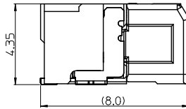
MATED WITH HEADER ASSEMBLY [REFERENCE]
