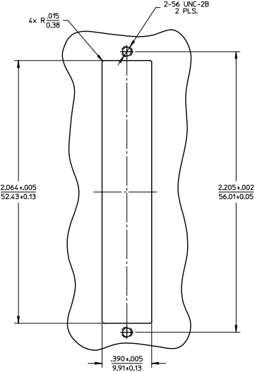
RECOMMENDED MOUNTING PATTERN
