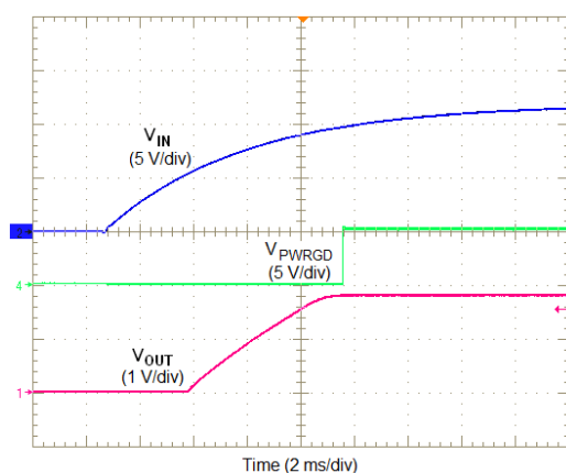
Figure 21. Start-Up Waveforms
