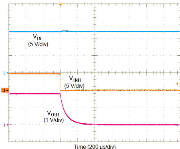
Figure 24. Inhibit Turn-Off
