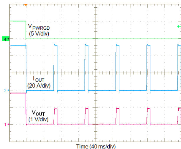
Figure 26. Overcurrent Limiting (Hiccup)
