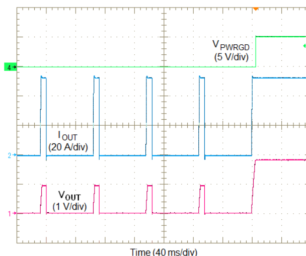
Figure 27. Removal of Overcurrent (Hiccup)
