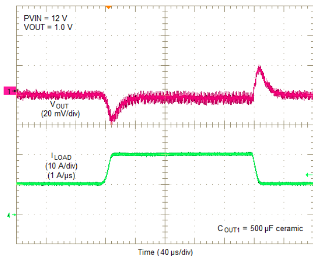
Figure 13. PV_{IN} = 12V , V_{OUT} = 1.0V , 10A Load Step
