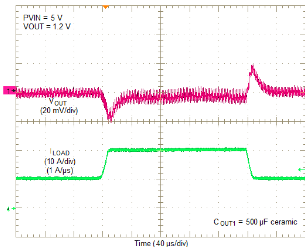
Figure 15. PV_{IN} = 5V , V_{OUT} = 1.2V , 10A Load Step
