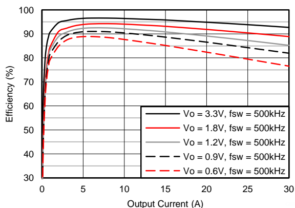
Figure 7. Efficiency vs. Output Current
