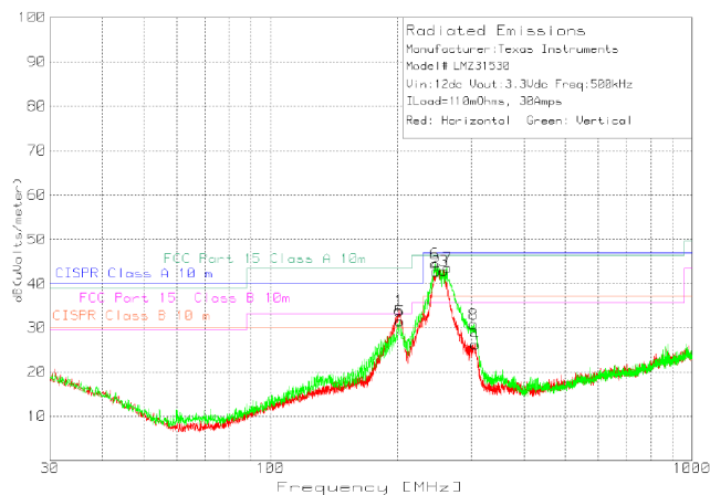
Figure 35. Radiated Emissions 12-V Input, 3.3-V Output, 30-A Load (EN55022 Class A)
