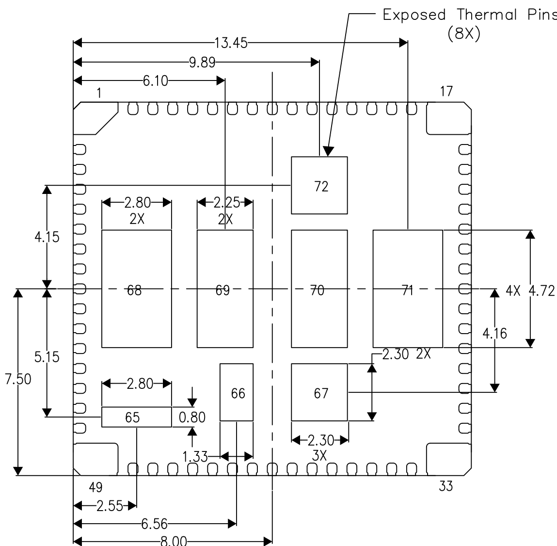
Bottom View Exposed Thermal Pad Dimensions Thermal Pad Tolerance: \pm 0.10\text{mm}
