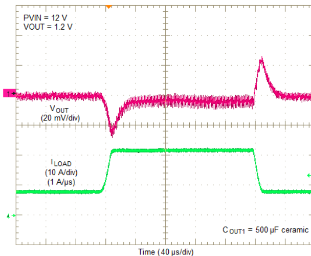
Figure 16. PV_{IN} = 12V , V_{OUT} = 1.2V , 5A Load Step
