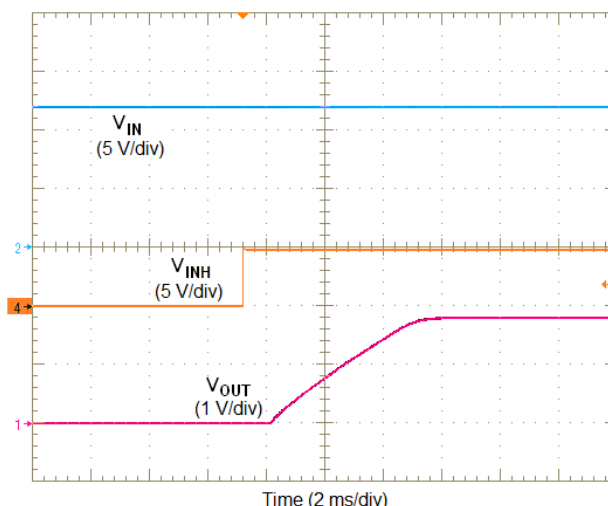
Figure 25. Inhibit Turn-On
