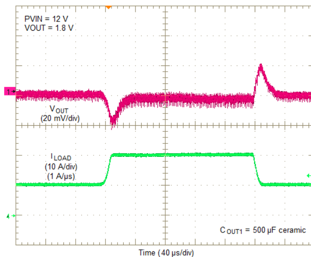
Figure 14. PV_{IN} = 12V , V_{OUT} = 1.8V , 10A Load Step
