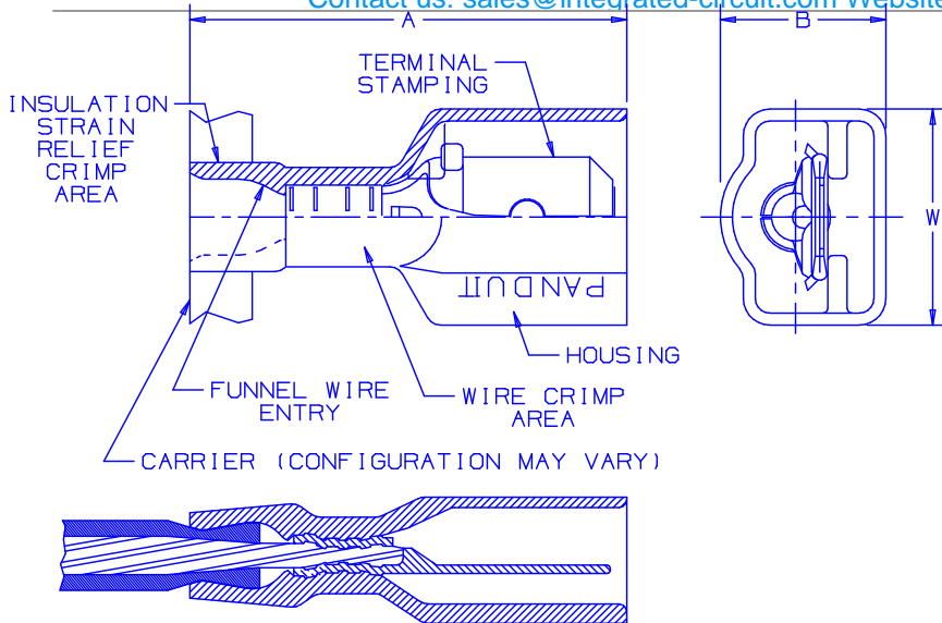
SECTION VIEW OF CRIMPED DISCONNECT
