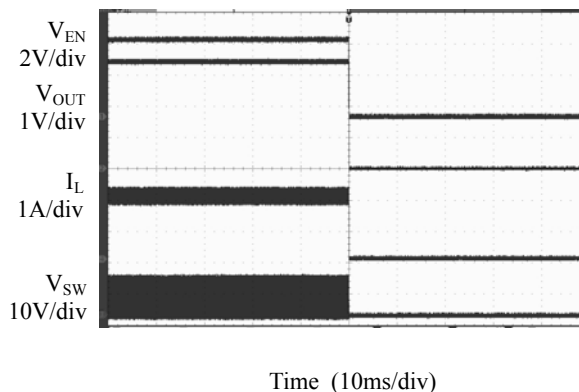
Figure 11. Enable Turn off Characteristic ( I_{\text{OUT}}=2\text{A} , CC Mode)
