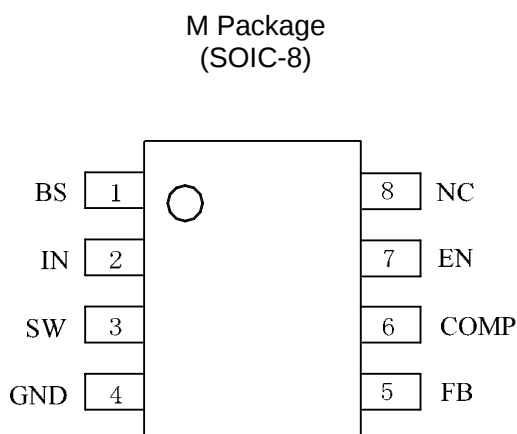
Figure 2. Pin Configuration of AP3202 (Top View)
