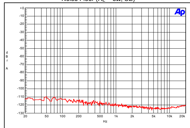
Noise Floor ( R_L = 8\Omega , SE)
