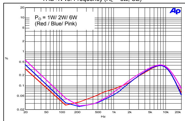
THD+N vs. Frequency ( R_L = 8\Omega , SE)
