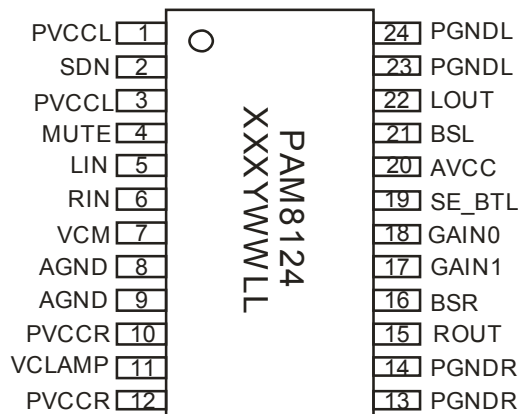
TSSOP-24-EP
