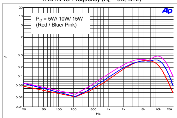
THD+N vs. Frequency ( R_L = 8\Omega , BTL)
