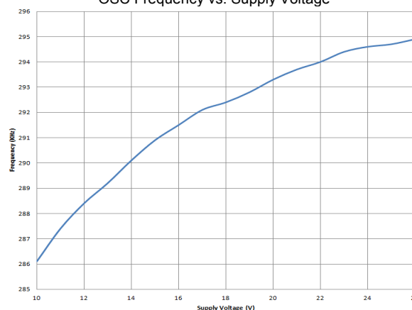
OSC Frequency vs. Supply Voltage
