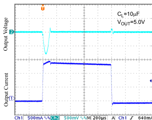
Figure 13. Load Transient
