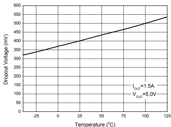
Figure 5. Dropout Voltage vs. Temperature
