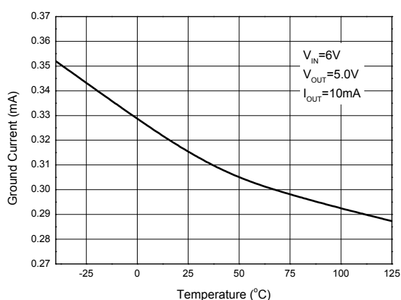
Figure 9. Ground Current vs. Temperature
