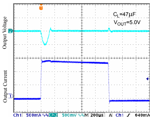
Figure 14. Load Transient
