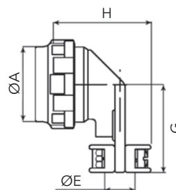
90° cable clamp (Type 92)
