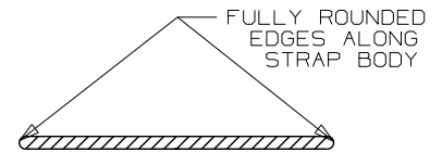
SECTION A - A SCALE 8:1
