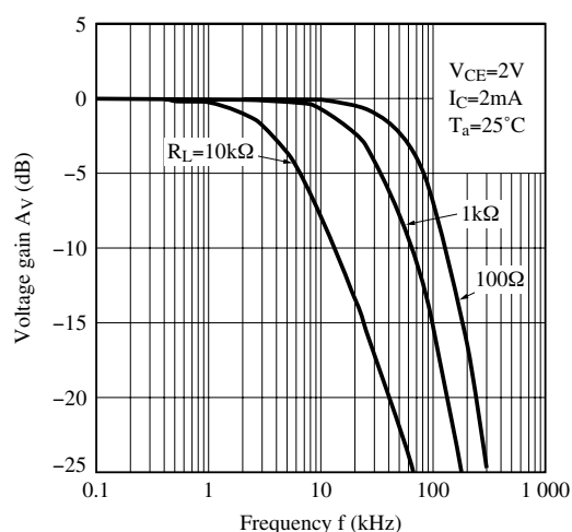
Fig.16 Frequency Response
