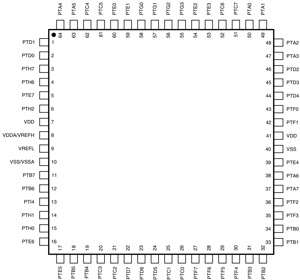
Figure 22. 64-pin QFP/LQFP packages
