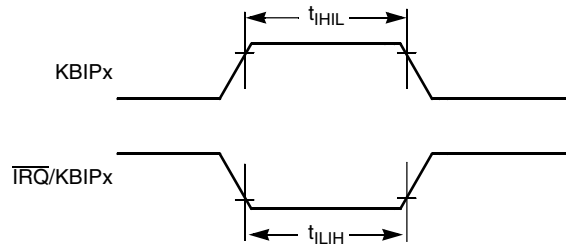
Figure 10. KBIPx timing
