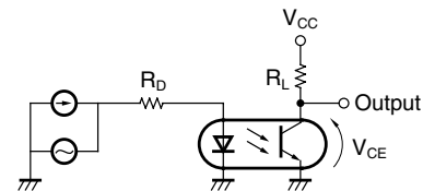
Fig.16 Test Circuit for Frequency Response
