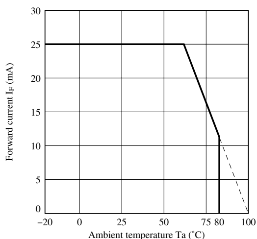
Fig.8 Forward Current vs. Ambient Temperature
