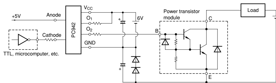
Fig.24 Application Circuit
