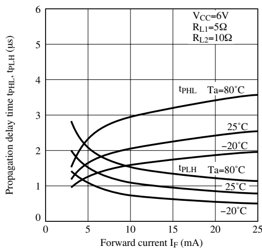
Fig.21 Propagation Delay Time vs. Forward Current
