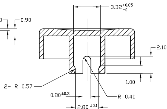
SECTION B-B DETAIL
