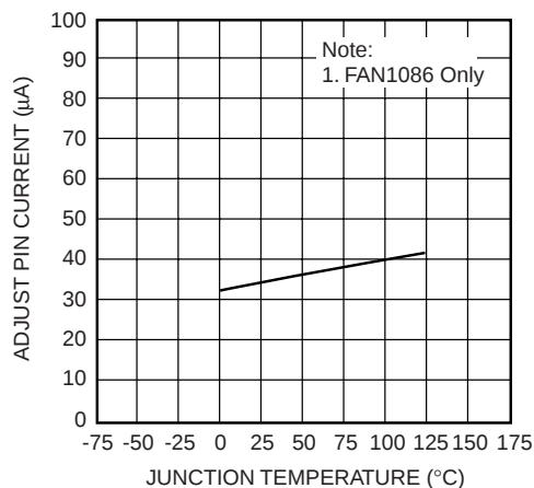
Figure 6. Adjust Pin Current vs. Temperature
