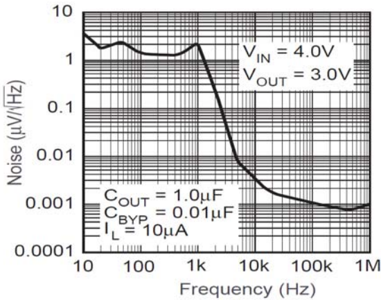
Figure 11. Noise Performance
