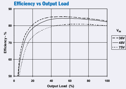
PT4854 Performance Characteristics (See Note A) ( I_{o1} = 10A, I_{o2} = 7.5A, I_{o3} = 7.5A represents 100% Load)
