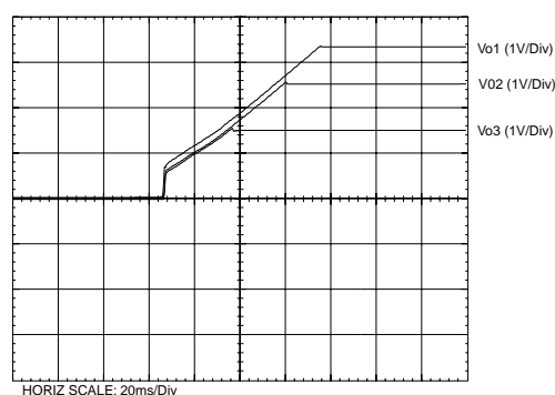
Figure 3; Vo1, Vo2, Vo3 Power-Up Sequence
