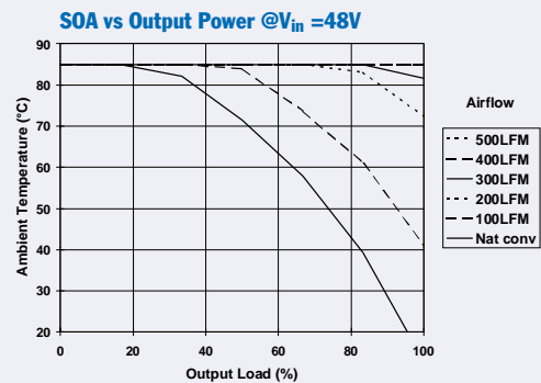
PT4854 Safe operating Area Curves (See Note B) ( I_{o1} + I_{o2} + I_{o3} = 25A , represents 100% load)
