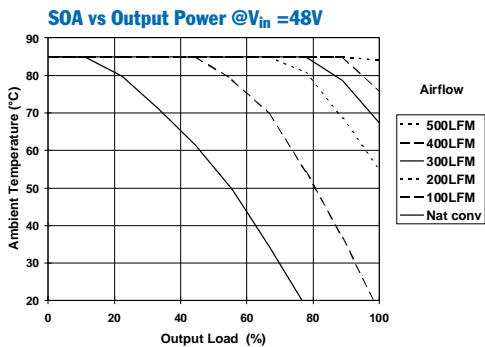
PT4851 Safe operating Area Curves (See Note B) ( I_{o1} + I_{o2} + I_{o3} = 25A , represents 100% load)
