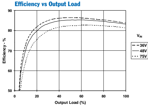
PT4853 Performance Characteristics (See Note A) ( I_{o1} = 10A, I_{o2} = 7.5A, I_{o3} = 7.5A represents 100% Load)
