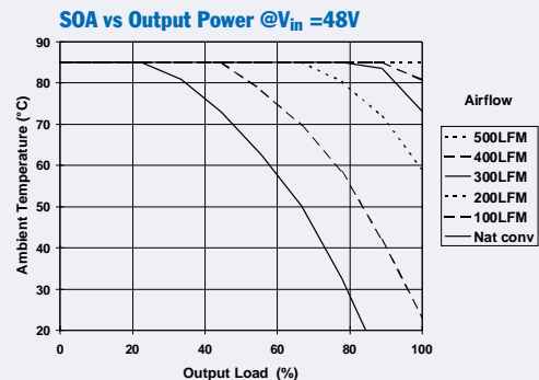
PT4852 Safe operating Area Curves (See Note B) ( I_{o1} + I_{o2} + I_{o3} = 25A , represents 100% load)
