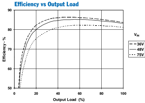
PT4851 Performance Characteristics (See Note A) ( I_{o1} = 10A, I_{o2} = 7.5A, I_{o3} = 7.5A represents 100% Load)
