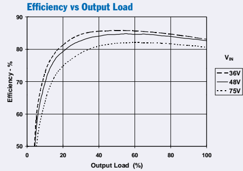
PT4852 Performance Characteristics (See Note A) ( I_{o1} = 10A, I_{o2} = 7.5A, I_{o3} = 7.5A represents 100% Load)
