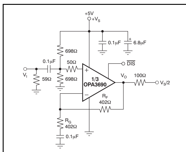
Figure 37. AC-Coupled, G = +2, Single-Supply Specification and Test Circuit
