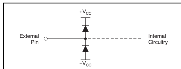
Figure 54. Internal ESD Protection
