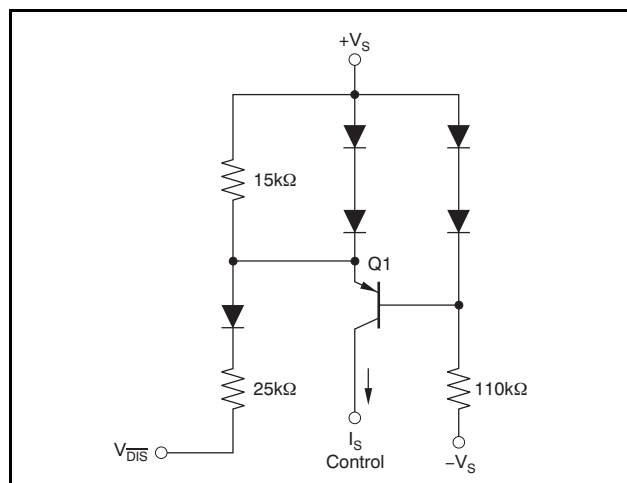
Figure 52. Simplified Disable Control Circuit
