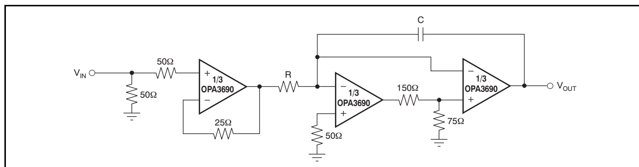
Figure 45. Wideband Integrator
