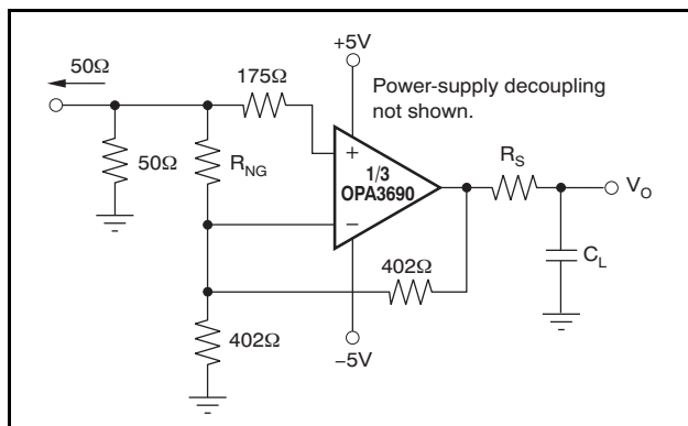
Figure 48. Capacitive Load Driving with Noise Gain Tuning
