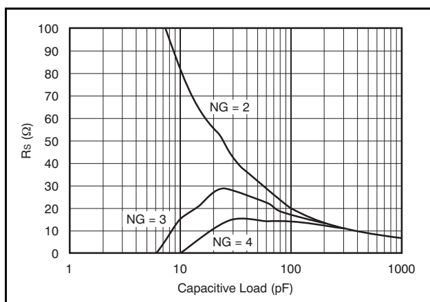
Figure 49. Required R_S vs Noise Gain
