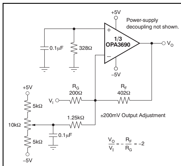
Figure 51. DC-Coupled, Inverting Gain of –2, with Offset Adjustment
