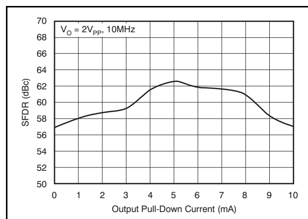
Figure 38. SFDR vs I_B
