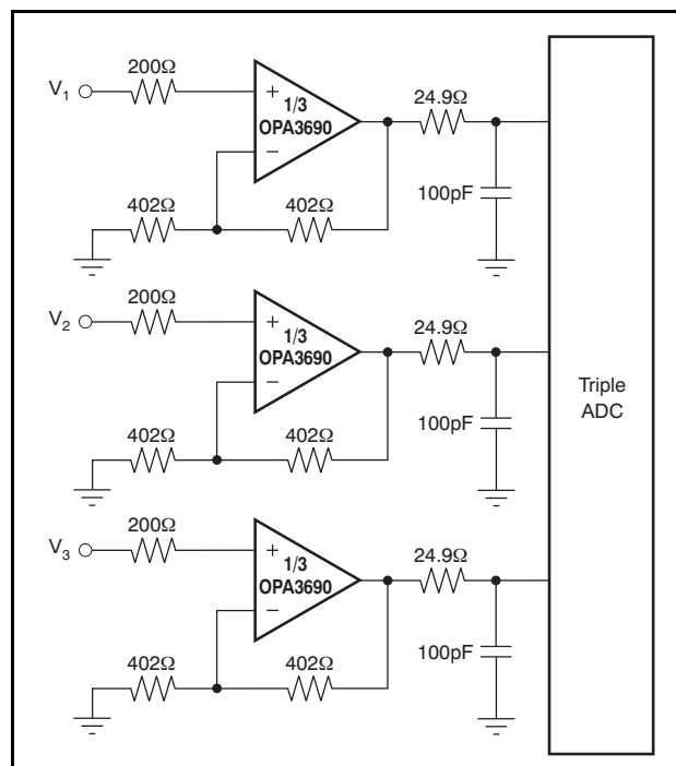
Figure 43. Triple ADC Driver
