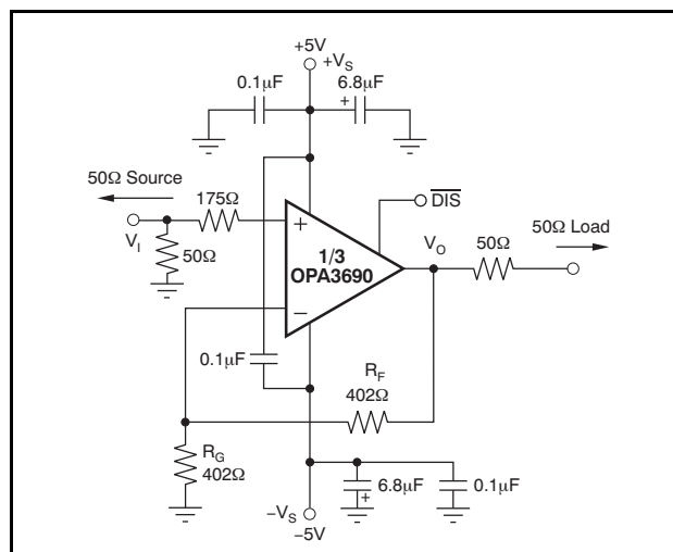
Figure 36. DC-Coupled, G = +2, Bipolar-Supply Specification and Test Circuit
