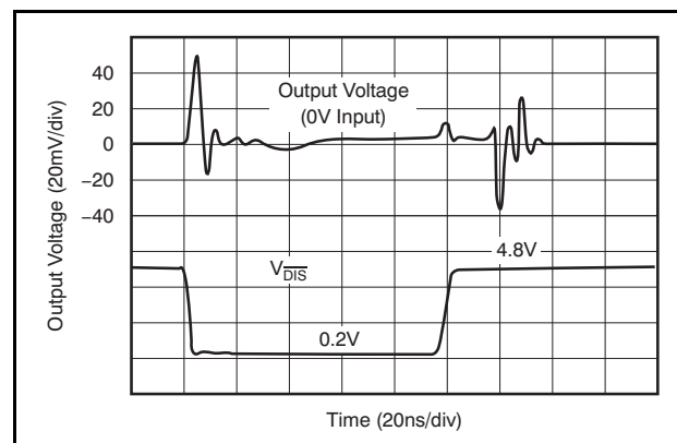
Figure 53. Disable/Enable Glitch
