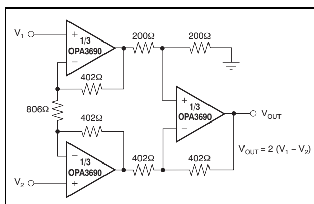
Figure 41. Instrumentation Amplifier
