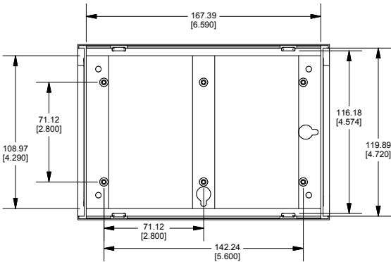
BOX - INSIDE VIEW
