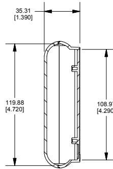
SECTION A-A END VIEW OF ASSEMBLY
