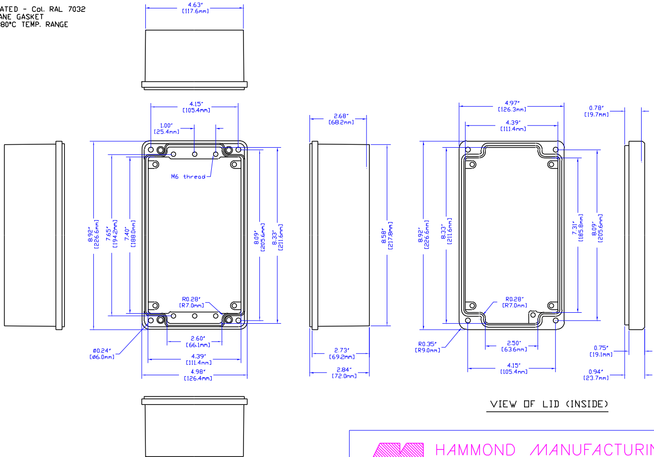
VIEW OF BOX (LID REMOVED)
