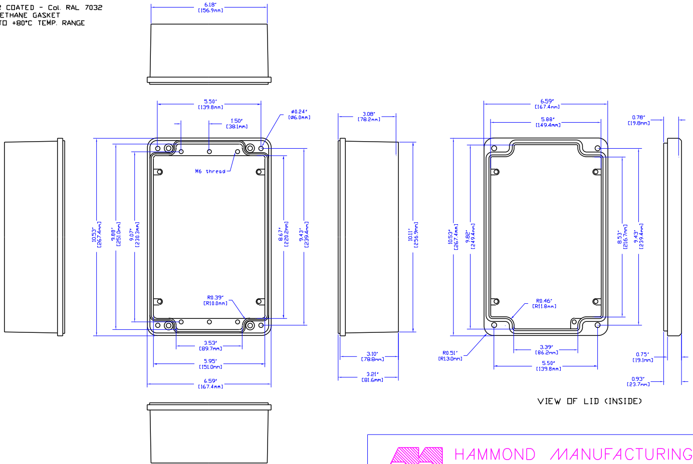
VIEW OF BOX (LID REMOVED)
