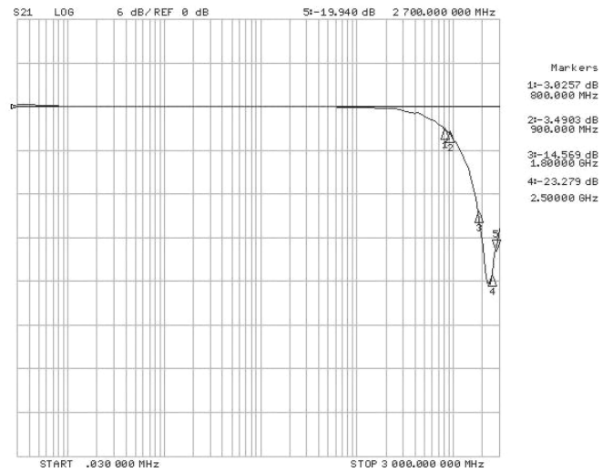
Typical Insertion Loss S21 (CLK Line)
