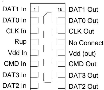
Figure 1 - Pin Identification and Configuration (Top Side View)
