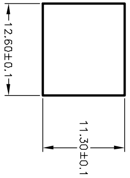
RECOMMENDED PANEL MOUNT
