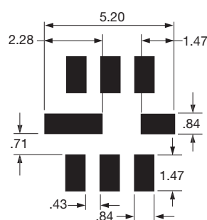
Figure 2) Land Pattern
