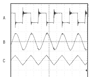
SWITCHING WAVEFORMS
