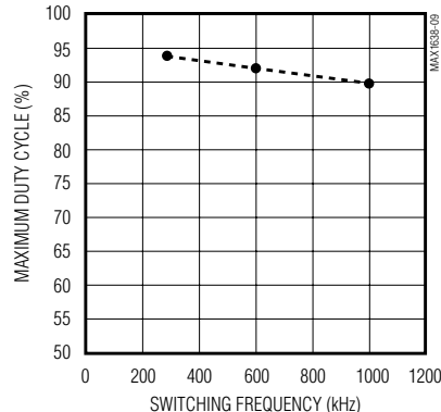
MAXIMUM DUTY CYCLE vs. SWITCHING FREQUENCY
