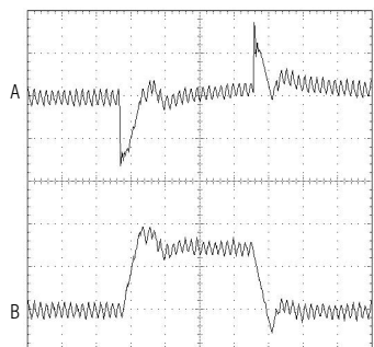
LOAD-TRANSIENT RESPONSE WITHOUT GLITCHCATCHER (C OUT = 440μF)
