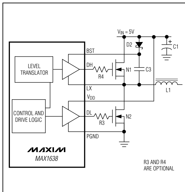
Figure 3. Boost Supply for Gate Drivers
