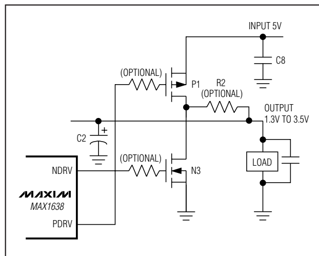
Figure 6. GlitchCatcher Circuit
