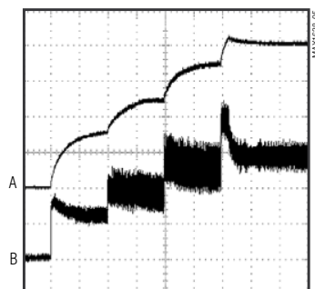
STARTUP WAVEFORMS
