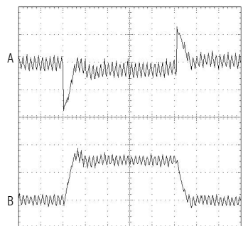
LOAD-TRANSIENT RESPONSE WITHOUT GLITCHCATCHER (C OUT = 880μF)
