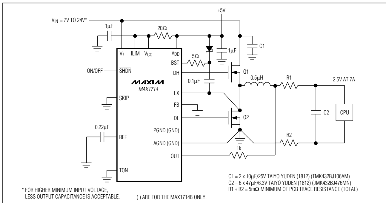
Figure 7. All-Ceramic-Capacitor Application
