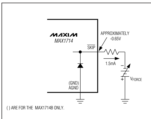
Figure 6. Disabling Over/Undervoltage Protection (No-Fault Test Mode)
