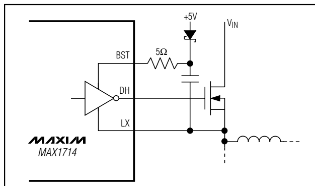
Figure 5. Reducing the Switching-Node Rise Time
