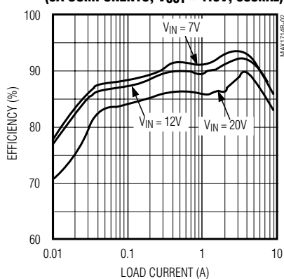
EFFICIENCY vs. LOAD CURRENT (8A COMPONENTS, V_{OUT} = 1.6V , 300kHz)
