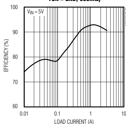
EFFICIENCY vs. LOAD CURRENT (1.5A COMPONENTS, V_{OUT} = 2.5V , T_{ON} = GND , 600kHz)
