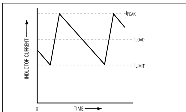
Figure 4. “Valley” Current-Limit Threshold Point
