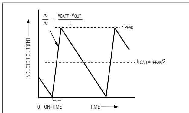
Figure 3. Pulse-Skipping/Discontinuous Crossover Point
