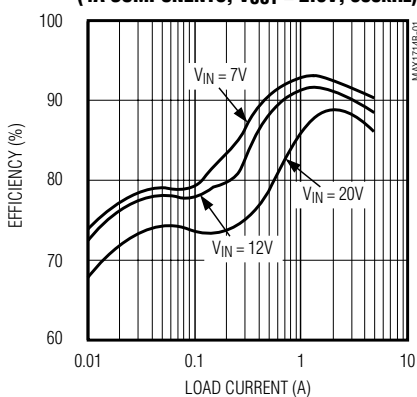
EFFICIENCY vs. LOAD CURRENT (4A COMPONENTS, V_{OUT} = 2.5V , 300kHz)
