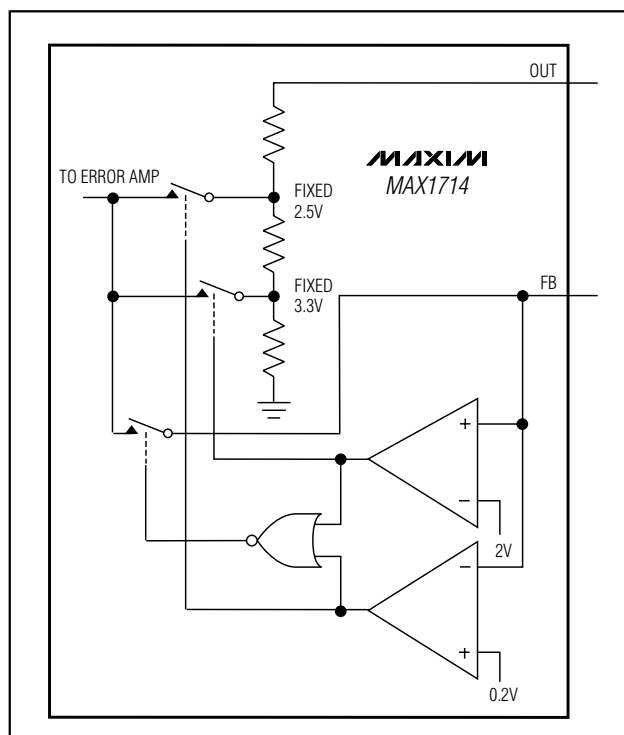
Figure 8. Feedback Mux
