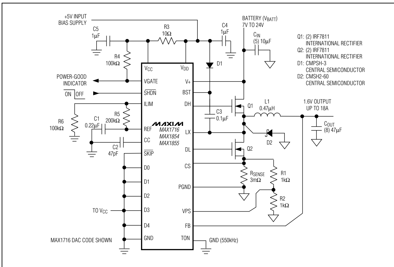
Figure 13. All-Ceramic-Capacitor Application (Circuit #4)
