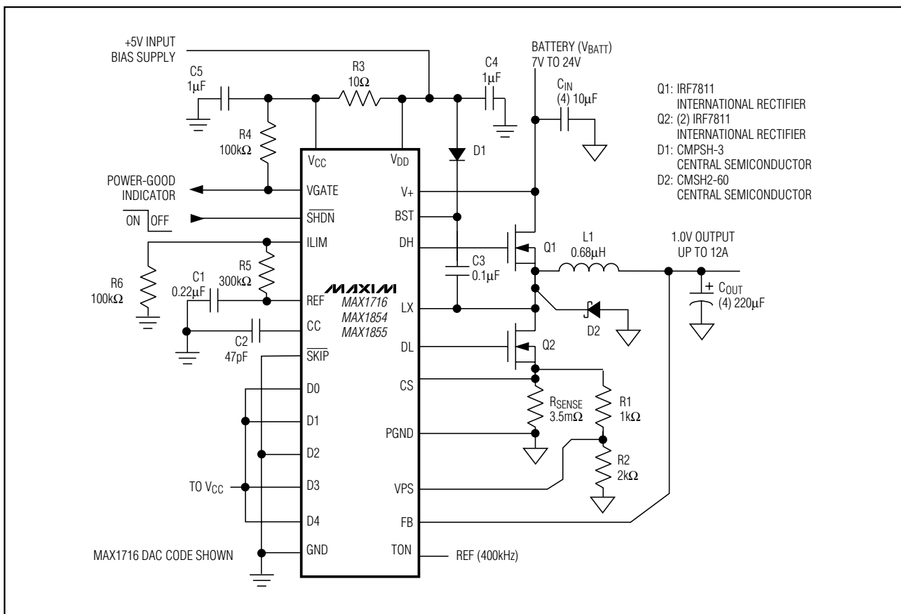
Figure 12. Low-Voltage Application (Circuit #3)
