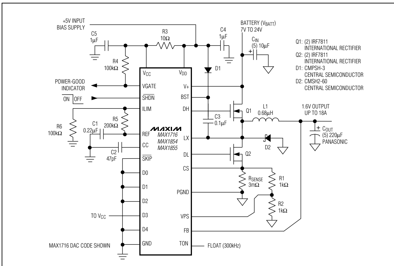
Figure 1. Standard High-Power Application (Circuit #1)
