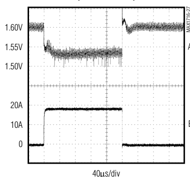
LOAD-TRANSIENT RESPONSE ( V_{BATT} = 4.5\text{V} )
