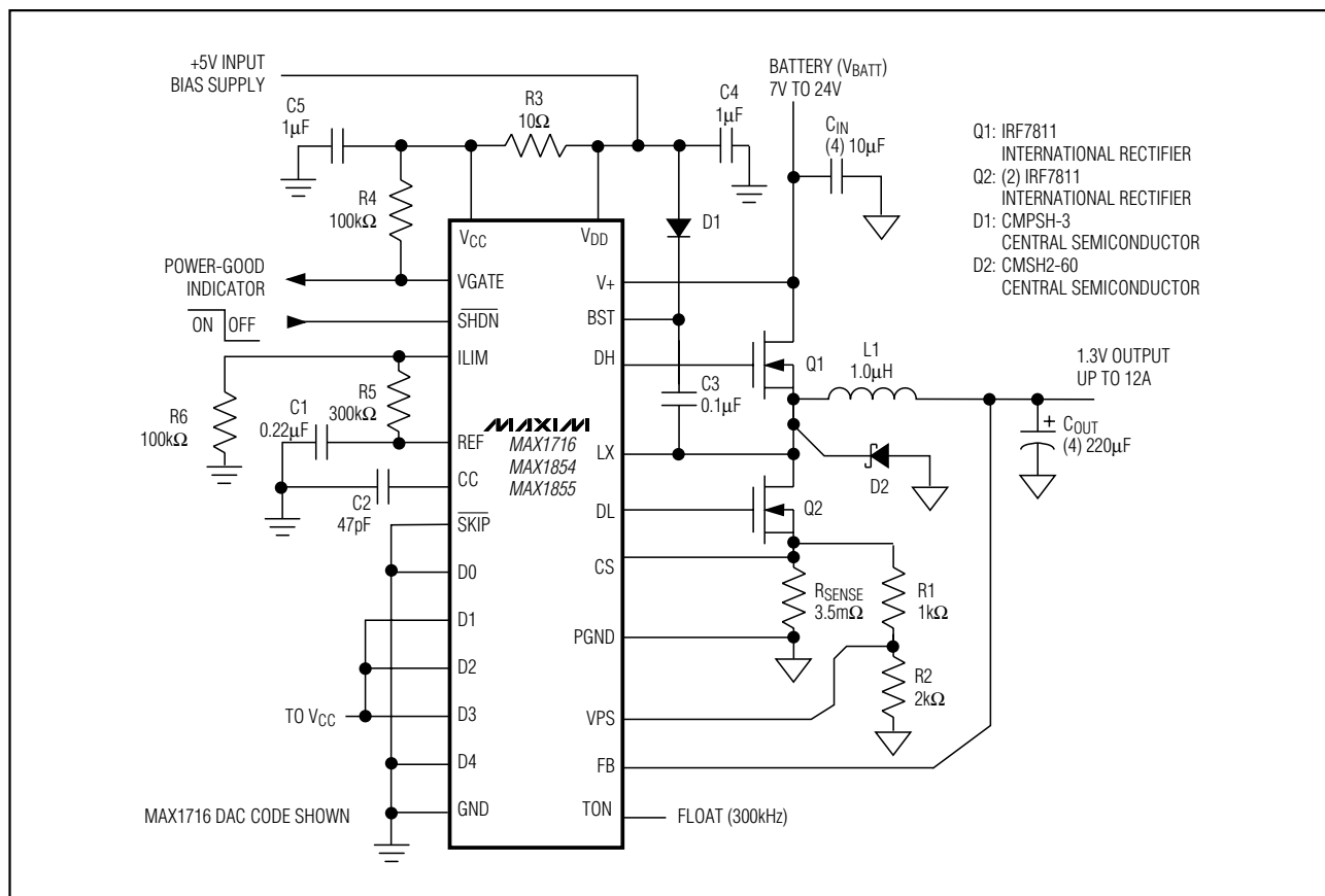
Figure 11. Low-Current Application (Circuit #2)
