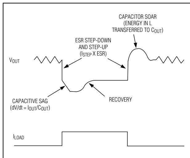
Figure 8. Transient-Response Regions
