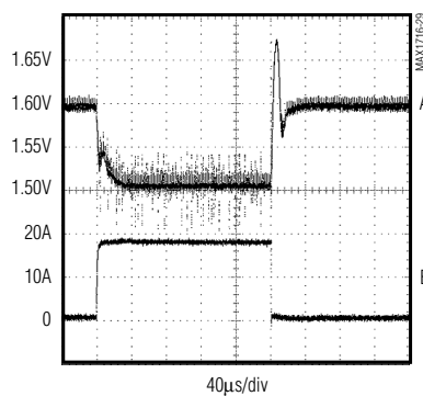
LOAD-TRANSIENT RESPONSE WITH CERAMIC OUTPUT CAPACITORS
