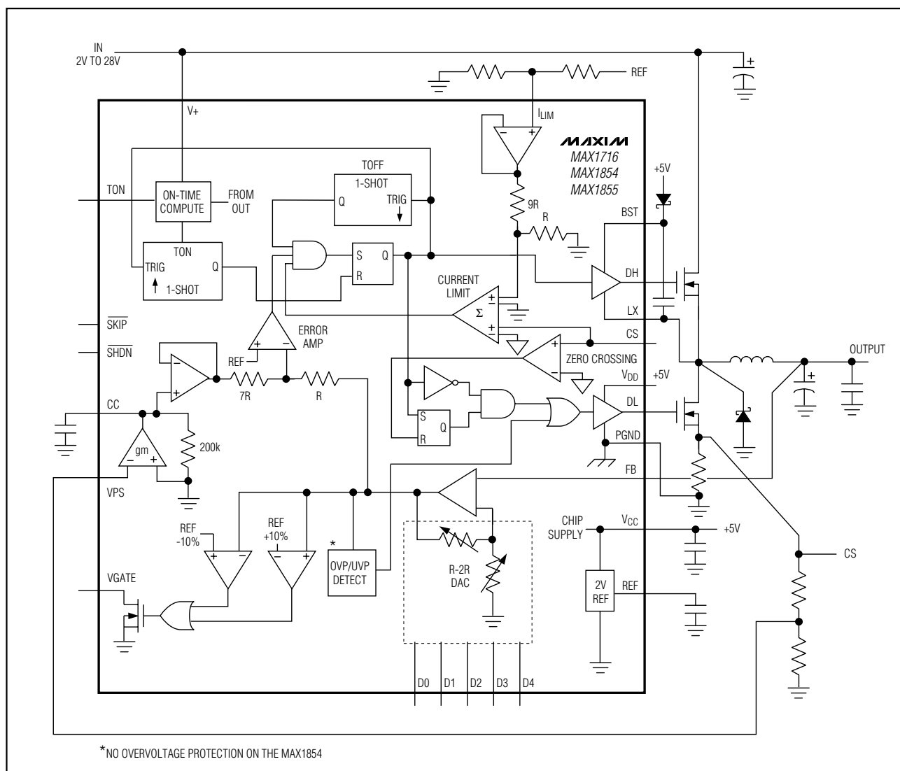
Figure 2. Functional Diagram
