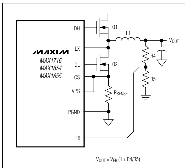
Figure 9. Adjusting V_{OUT} with a Resistor-Divider
