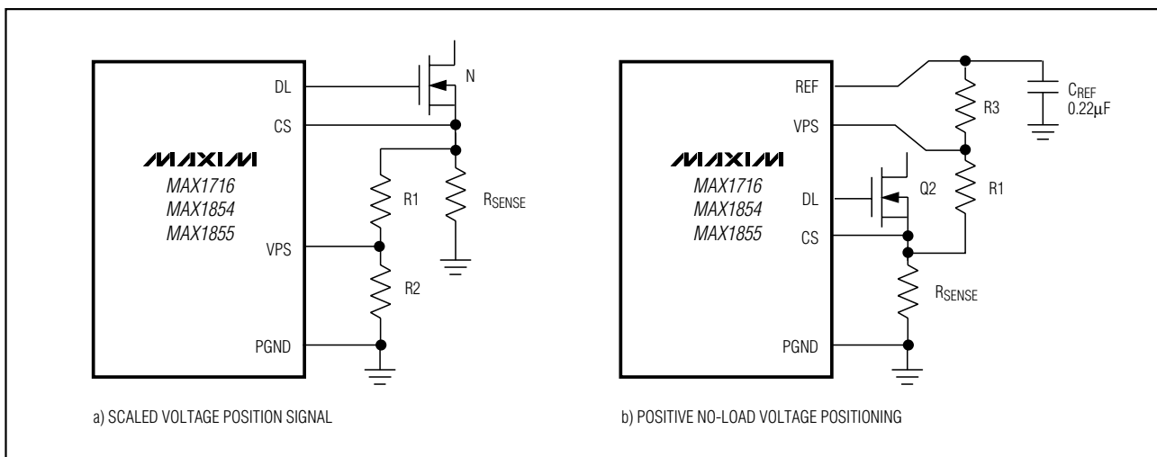
Figure 6. Voltage-Positioning Configurations
