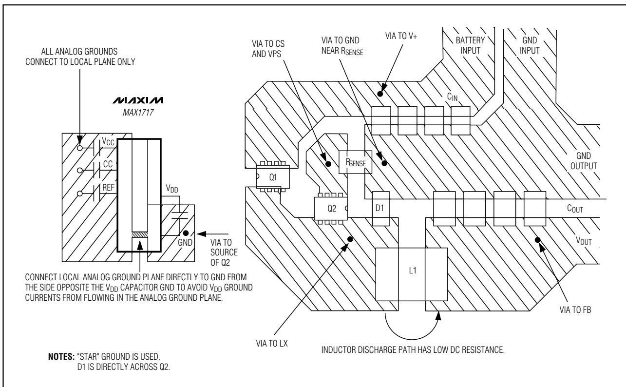
Figure 10. Power-Stage PC Board Layout Example
