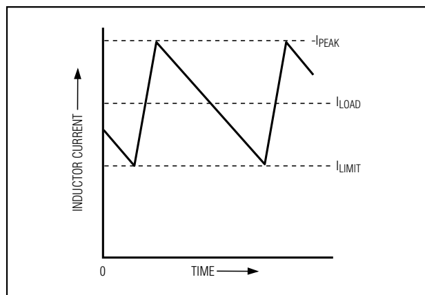
Figure 4. "Valley" Current-Limit Threshold Point
