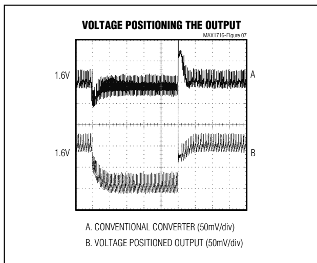
Figure 7. Voltage Positioning the Output
