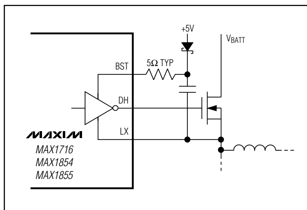
Figure 5. Reducing the Switching-Node Rise Time
