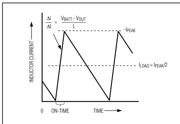
Figure 3. Pulse-Skipping/Discontinuous Crossover Point
